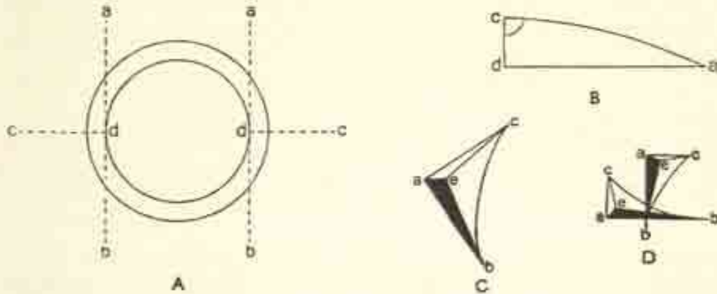
FIG. 6. Sections of reed and angles of wedges.
